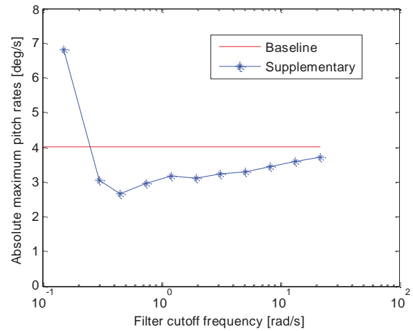
Figure 3 Maximum pitch rates across all above rated wind speeds
